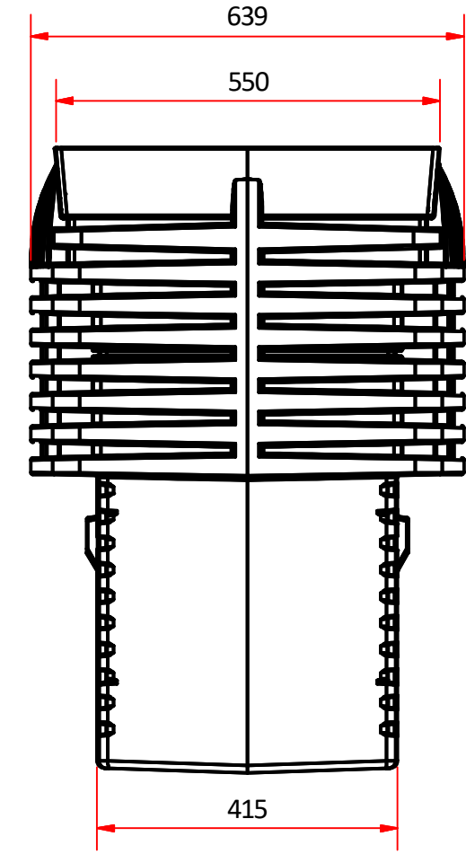
RH END VIEW ( 1:10 )
