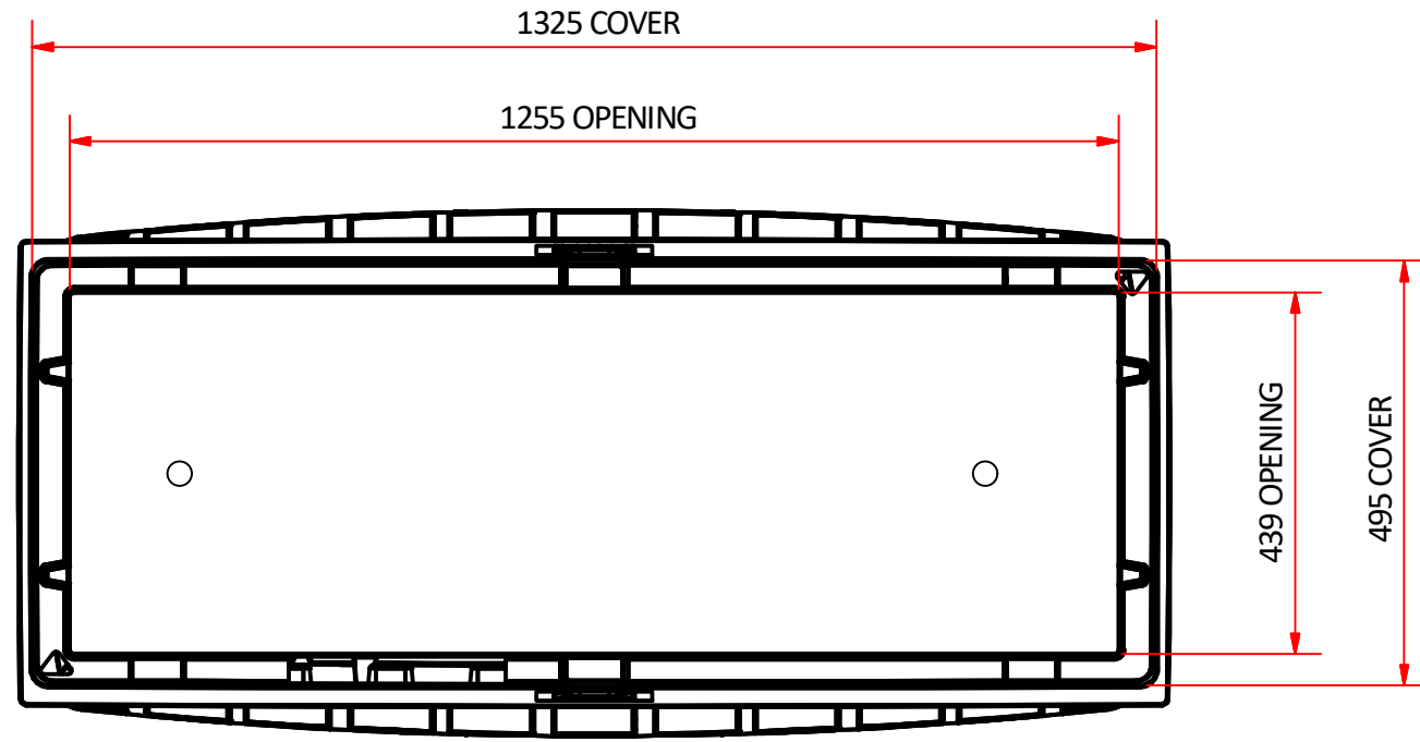
TOP VIEW ( 1:10 )
