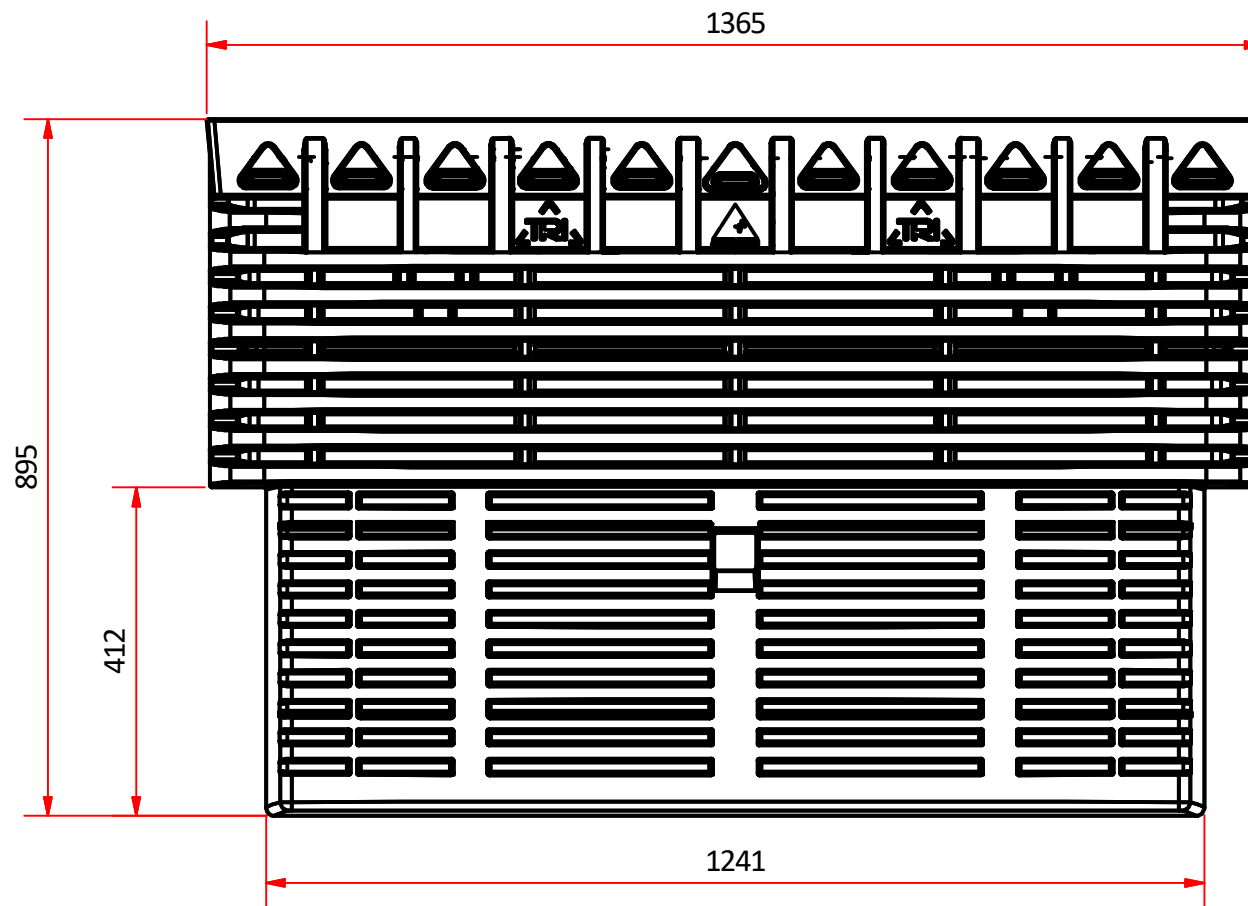
FRONT VIEW ( 1:10 )
